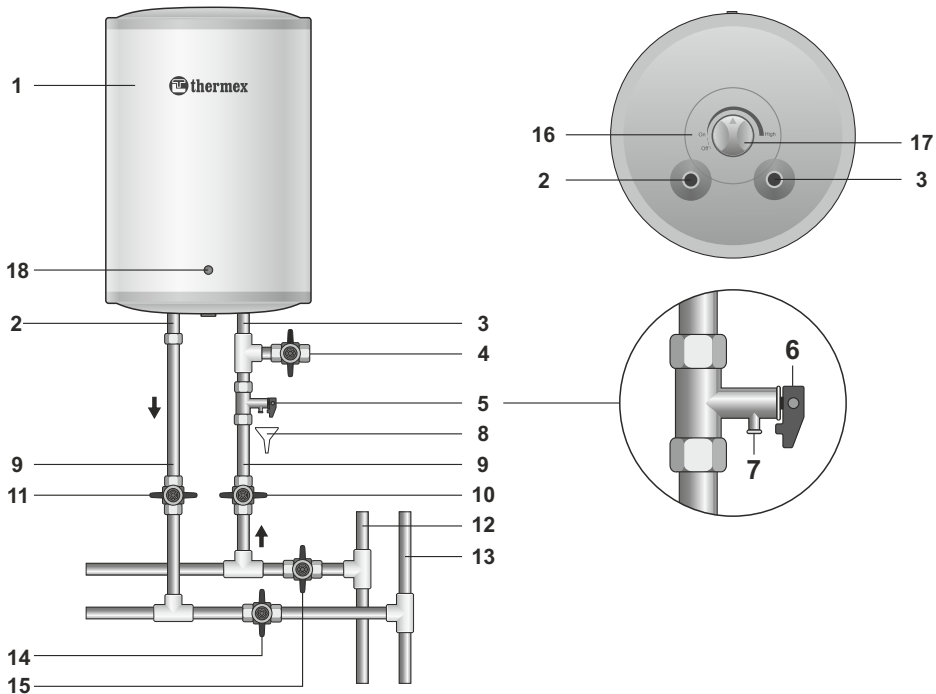
Fig. 1 Piping diagram and controls.
